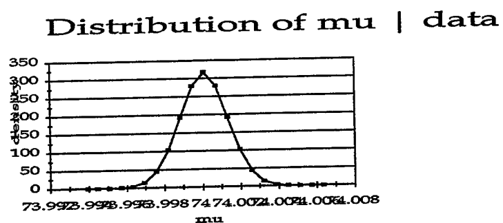
Figure 16: Plot of the posterior distribution for \mu|X for Example 3, after all 25 observations.
