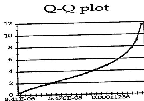
Figure 15: q - q plot of the sample variances against a \chi_4^2 for Example 3. Notice the poor fit. The R^2 for the associated regression is 0.85, which is highly significant against the Shapiro-Wilks criteria.
