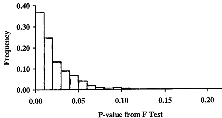
Figure 3. Histogram of P-Values for Test of H_0: \delta_1^2 = \delta_2^2 versus H_1: \delta_1^2 \neq \delta_2^2 .
