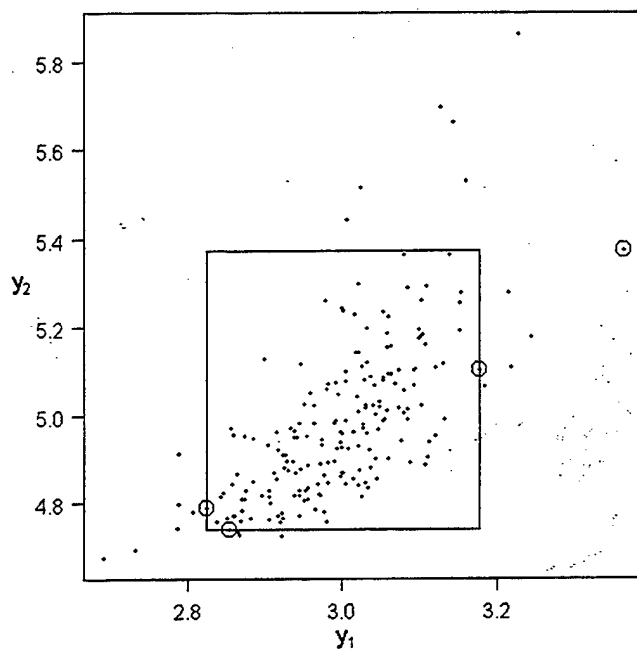
Figure 2. Overall Control Region for directions u_1, u_2, u_3 , and u_4
