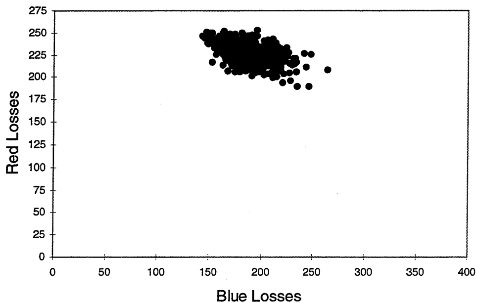
Figure 1. Scatterplot of Losses for Alternative 1
