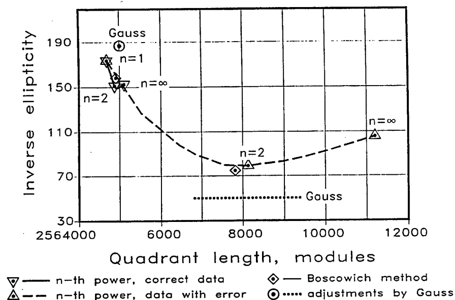
Figure 4. Adjustments by different methods.
