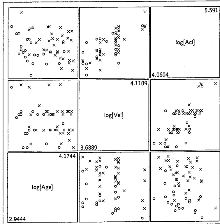
Figure 4: Scatterplot matrix of the transformed predictors in the collision data.
