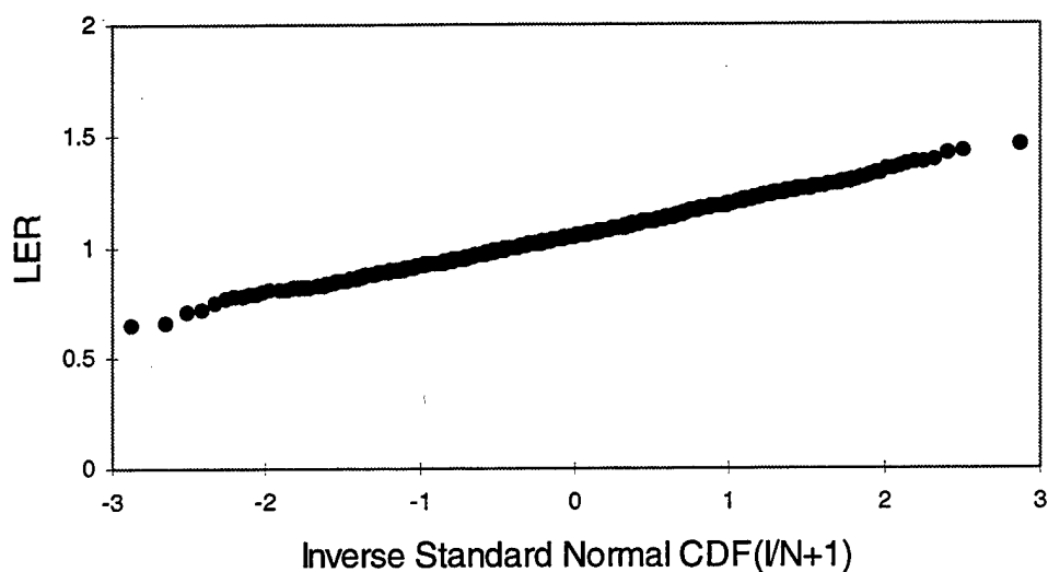
Figure 3. Quantile-Quantile Plot of LER for Alternative 1
