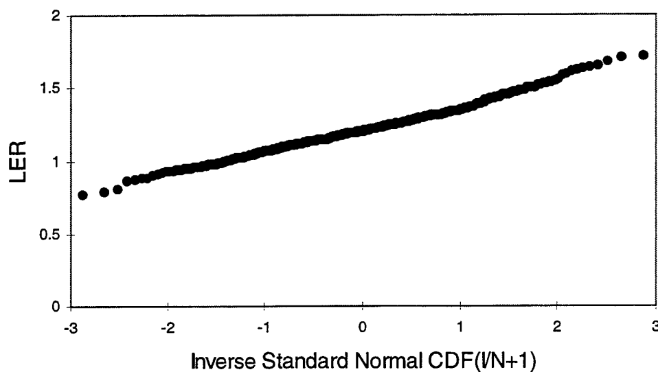
Figure 4. Quantile-Quantile Plot of LER for Alternative 2
