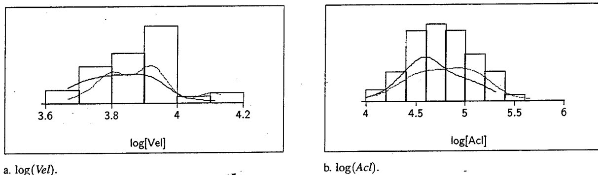
Figure 3: Density estimates of transformations of two predictors.
