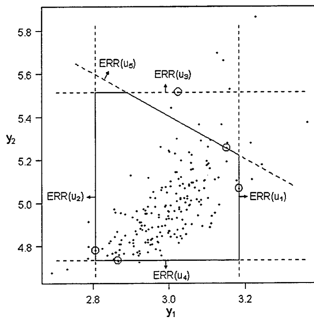
Figure 3. Overall Control Region for directions u_1, u_2, u_3, u_4 , and u_5
