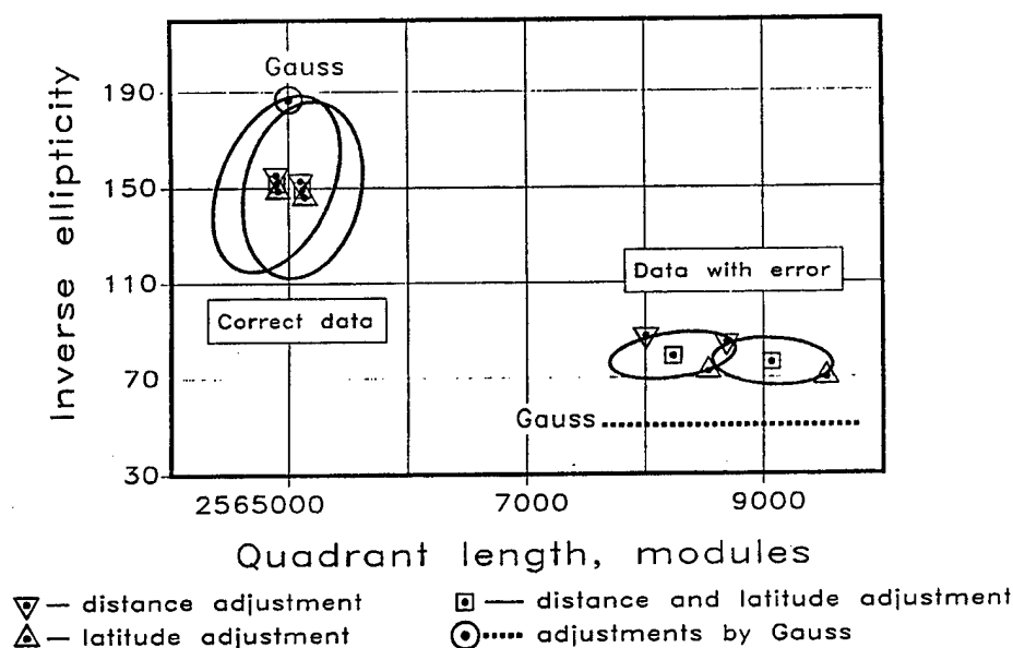
Figure 3. All least-squares adjustments.
