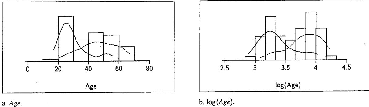
Figure 2: Density estimates of Age and \log(\text{Age}) for the collision data. These histograms are easier to compare using color; here the dark lines are for the deaths and the light lines are for the survivors. Throughout this paper, densities are estimated using a Gaussian kernel density estimate with bandwidth equal to 0.9 of the normal reference rule.
