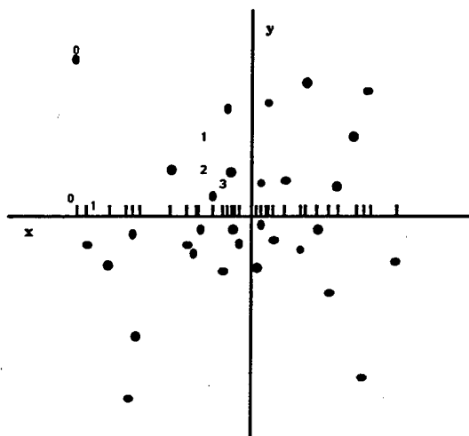
Figure 4. Mean Update Estimation of Mode.
