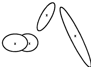
Figure 3. Random Binning for SIMEST.
