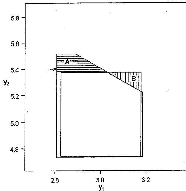
Figure 4. Comparison of the Controls Regions in Figures 3 and 4
