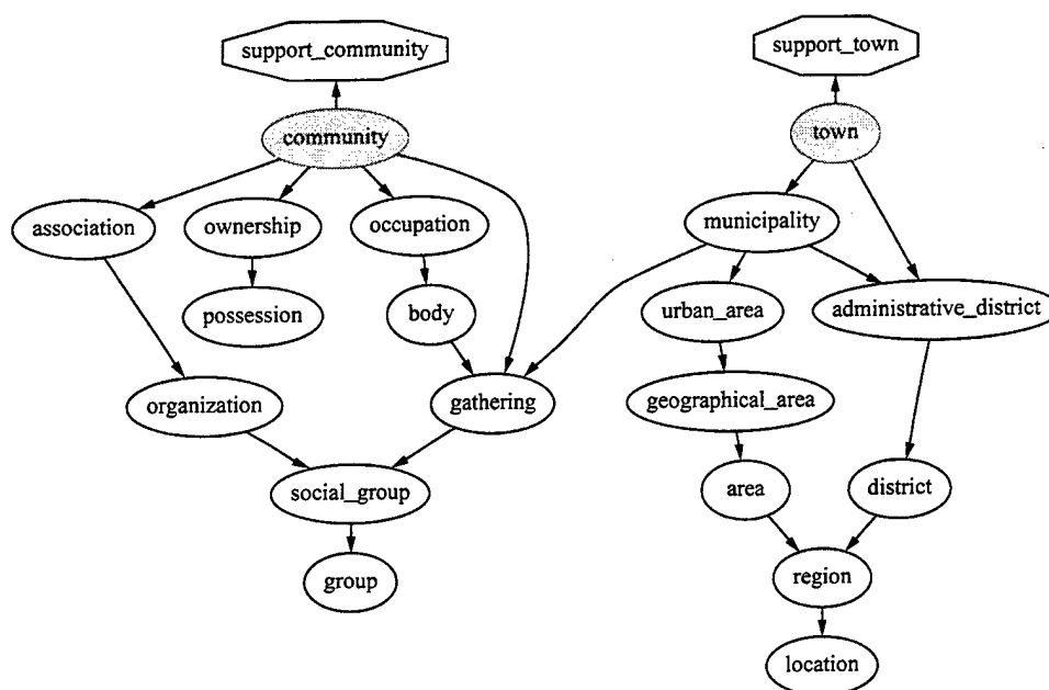
Figure 2: Word per node Bayesian network with hyponym→hypernym links
