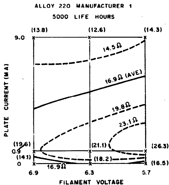
Fig. V - INTERFACE READING CONTOURS-TRIODES
