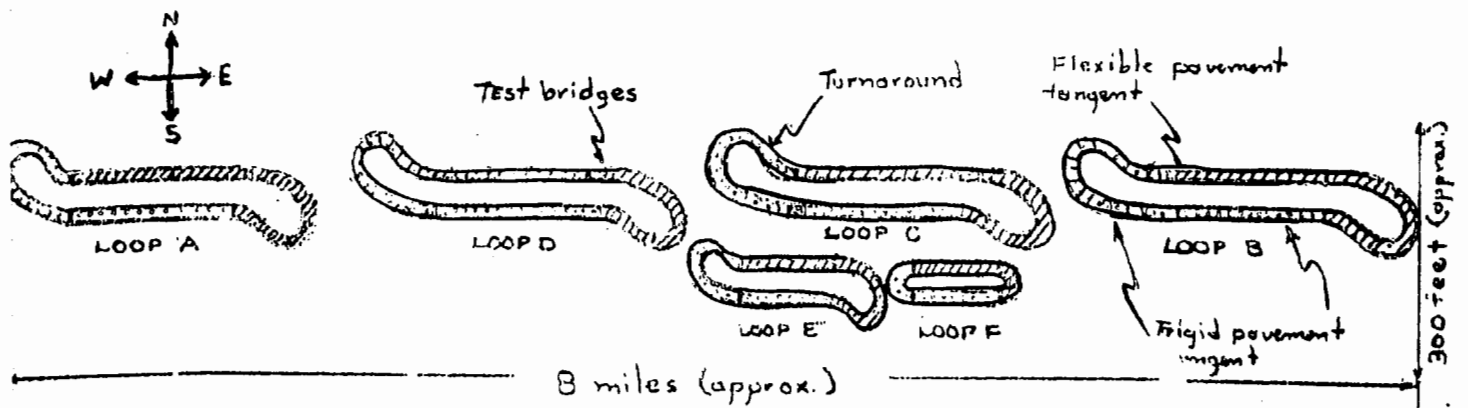
FIGURE 1: SCHEMATIC LOOP-TANGENT LAYOUT - AASHO TEST ROAD
