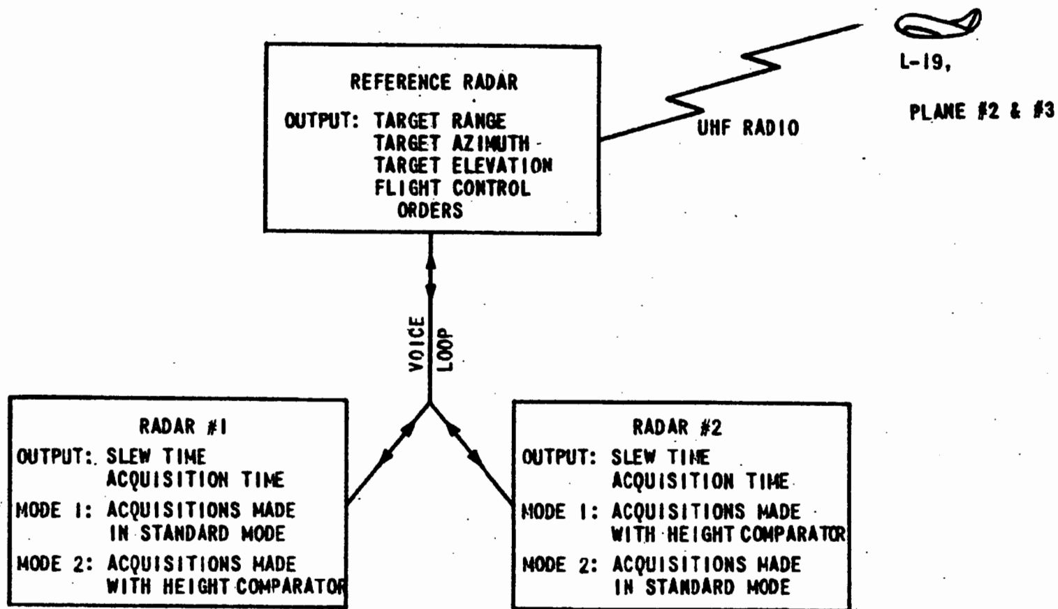
Fig 3 TEST CONFIGURATION
