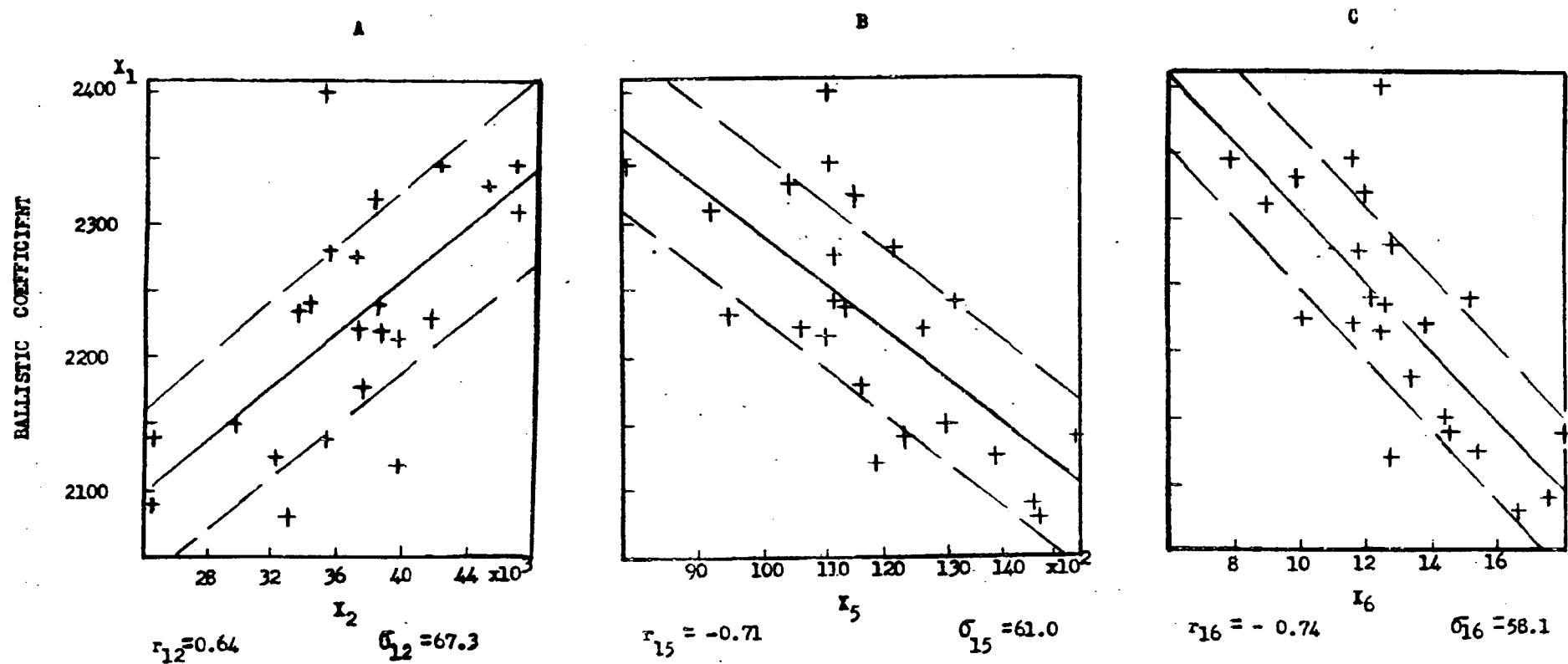
Figure 1. Scatter diagrams of gross relationship of yield strength ( X_2 ), area ( X_5 ), and per cent elongation ( X_6 ) for 23 specimens under stress-strain curve
