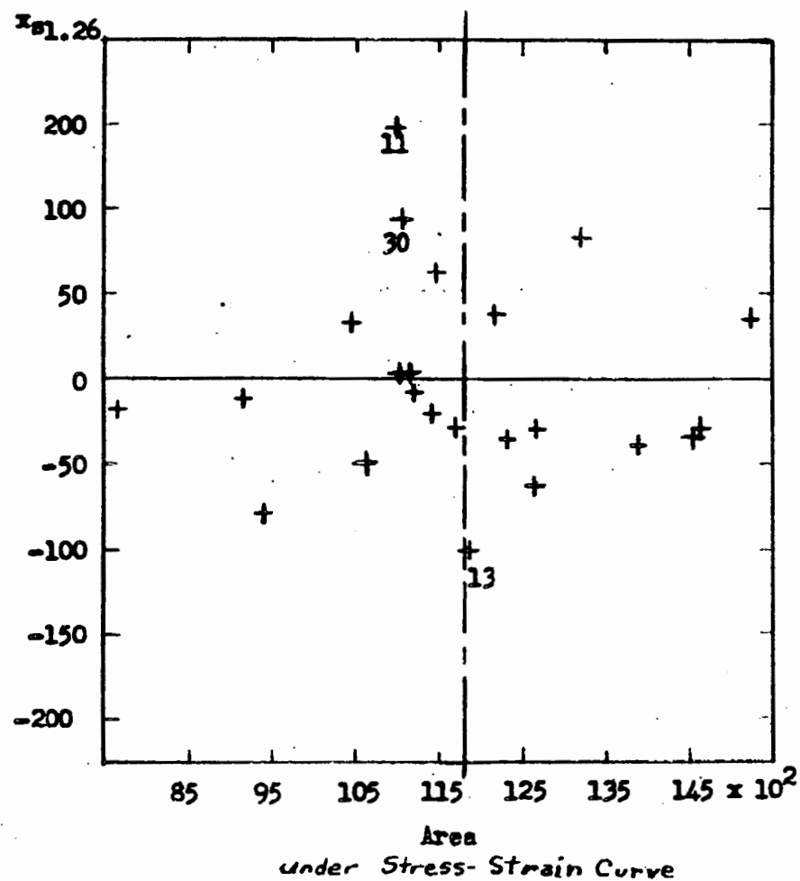
Figure 5. Scatter diagram of area 1 (X 5 ) and X 1 values adjusted for yield strength and percent elongation
