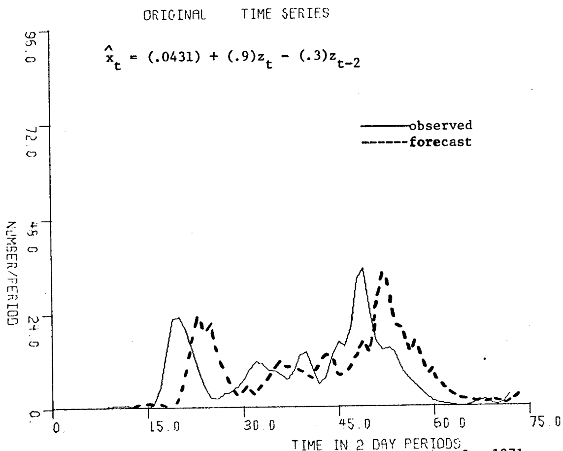
Fig. 6 Observed vs. 4-day ahead forecast series for 1971 smoothed data.
