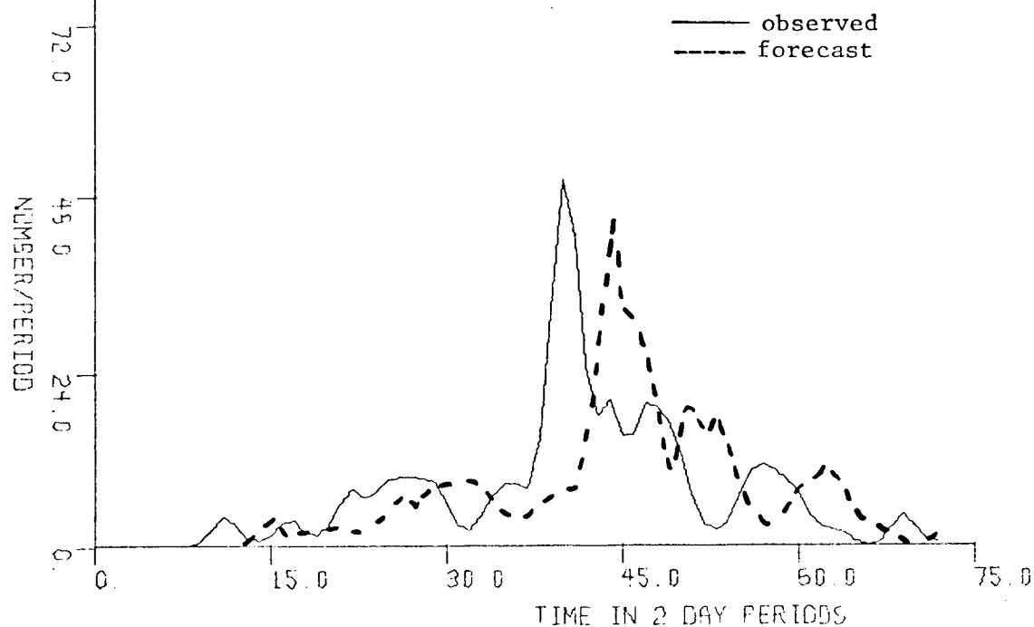
Fig. 4 Observed as 4-day ahead forecast series for 1969 smoothed data.
