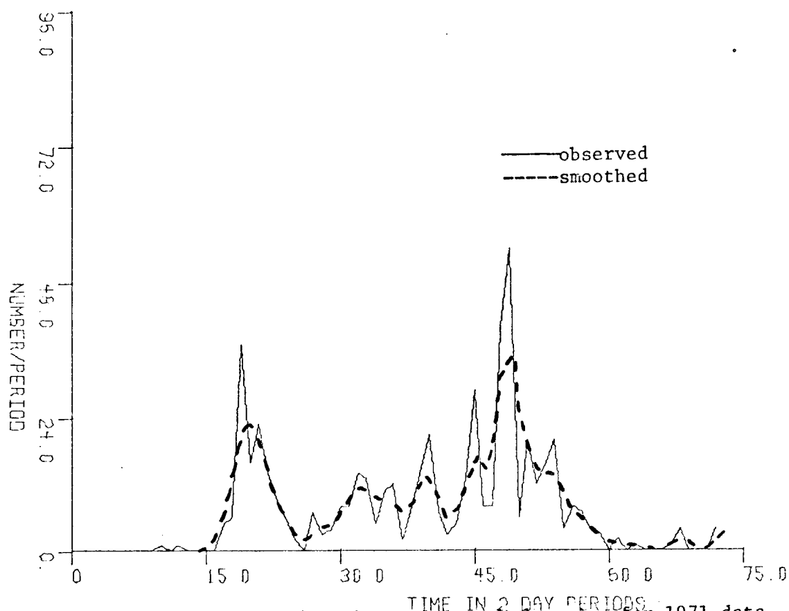
Fig. 3 Observed series vs. smoothed series for 1971 data.
