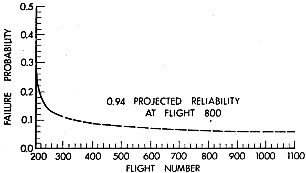
Figure 4. Projected Failure Probability Based on Flights 201 to 300.
