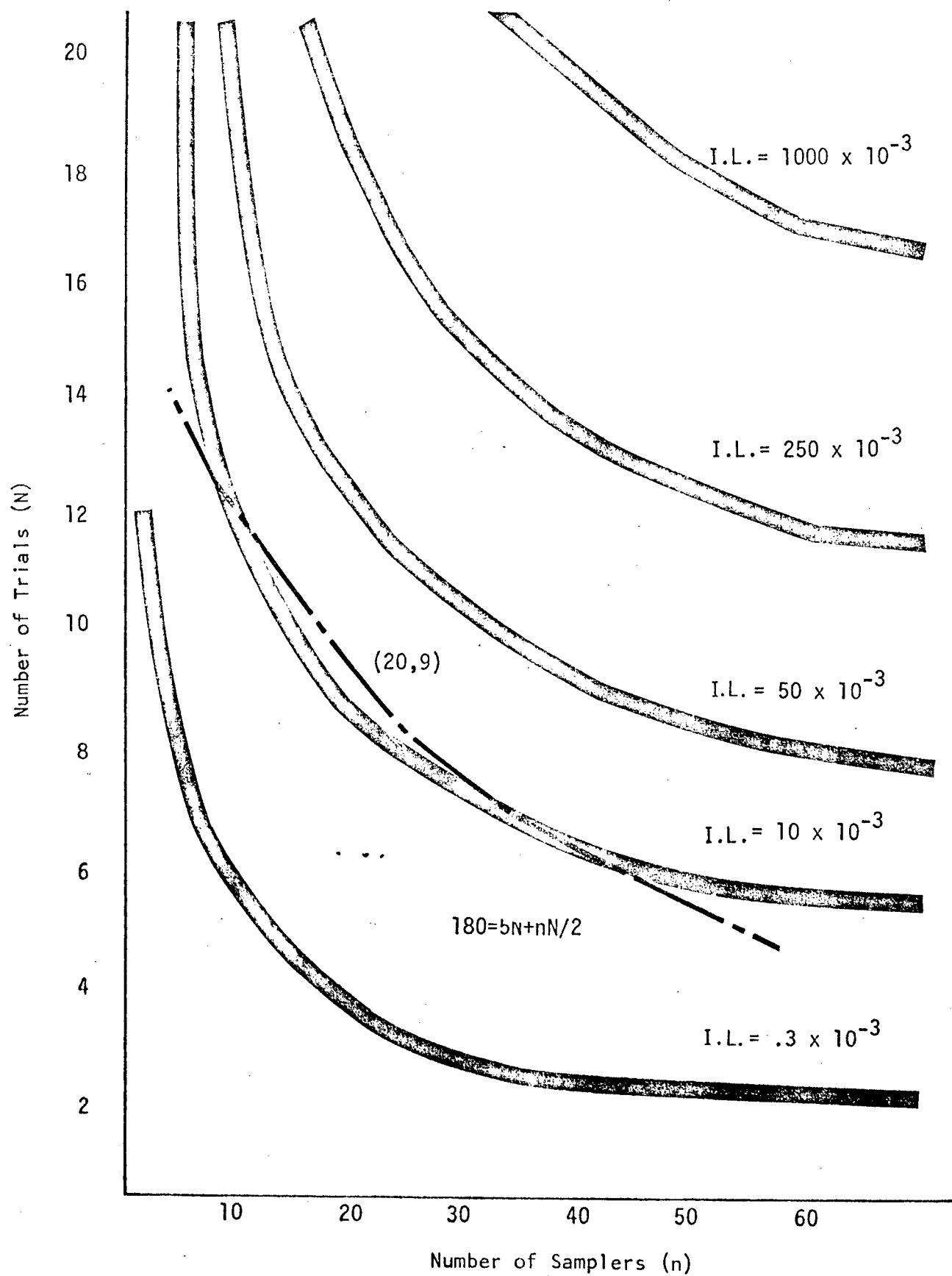
Figure 1. Information (I.L.) contours for varying values of n and N , and the selection of an optimal (N, N) combination
