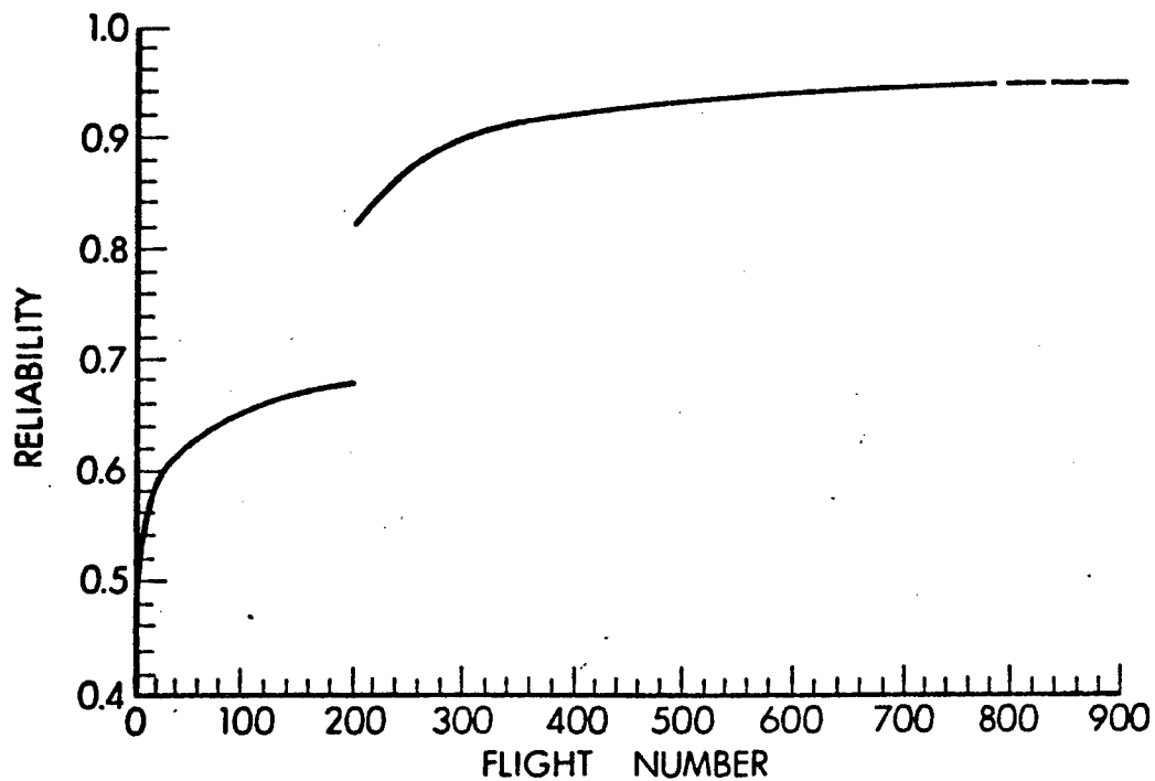
Figure 3. Estimated Reliability Based on Weibull Model.
