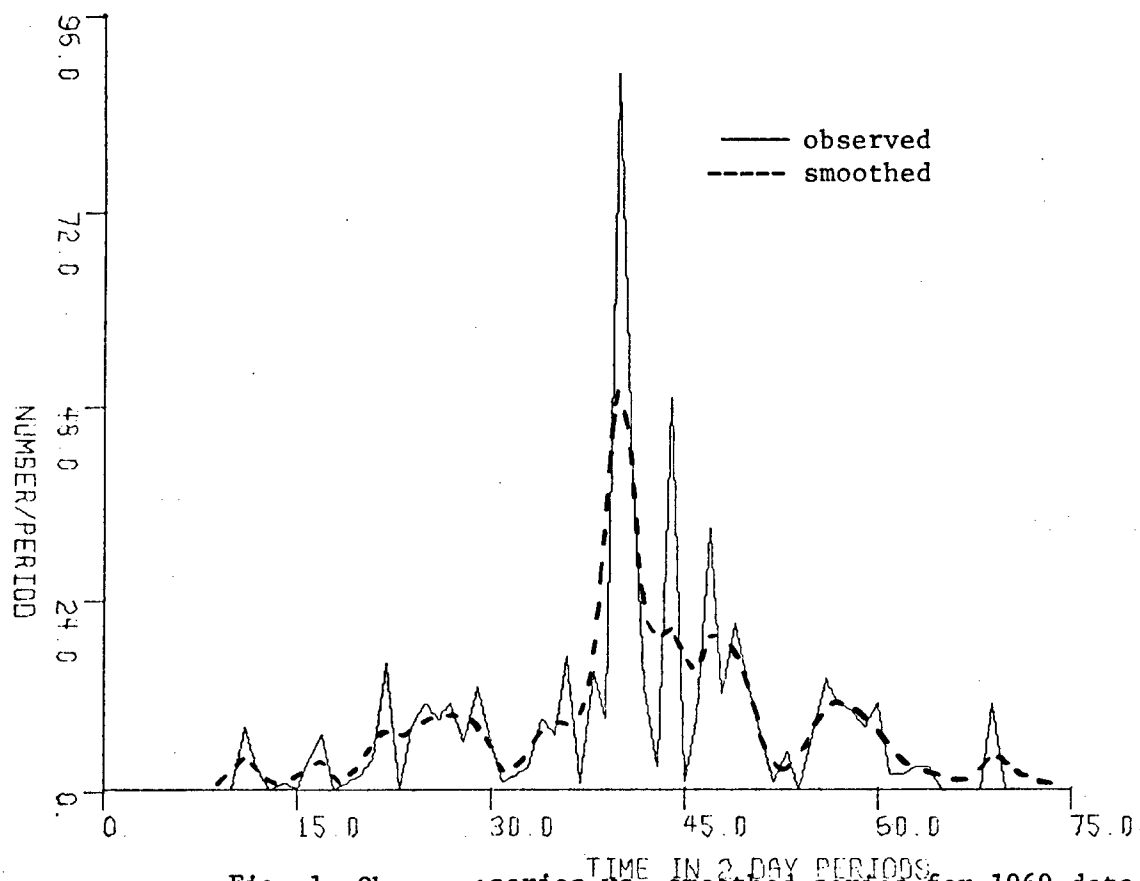
Fig. 1. Observed series vs. smoothed series for 1969 data.
