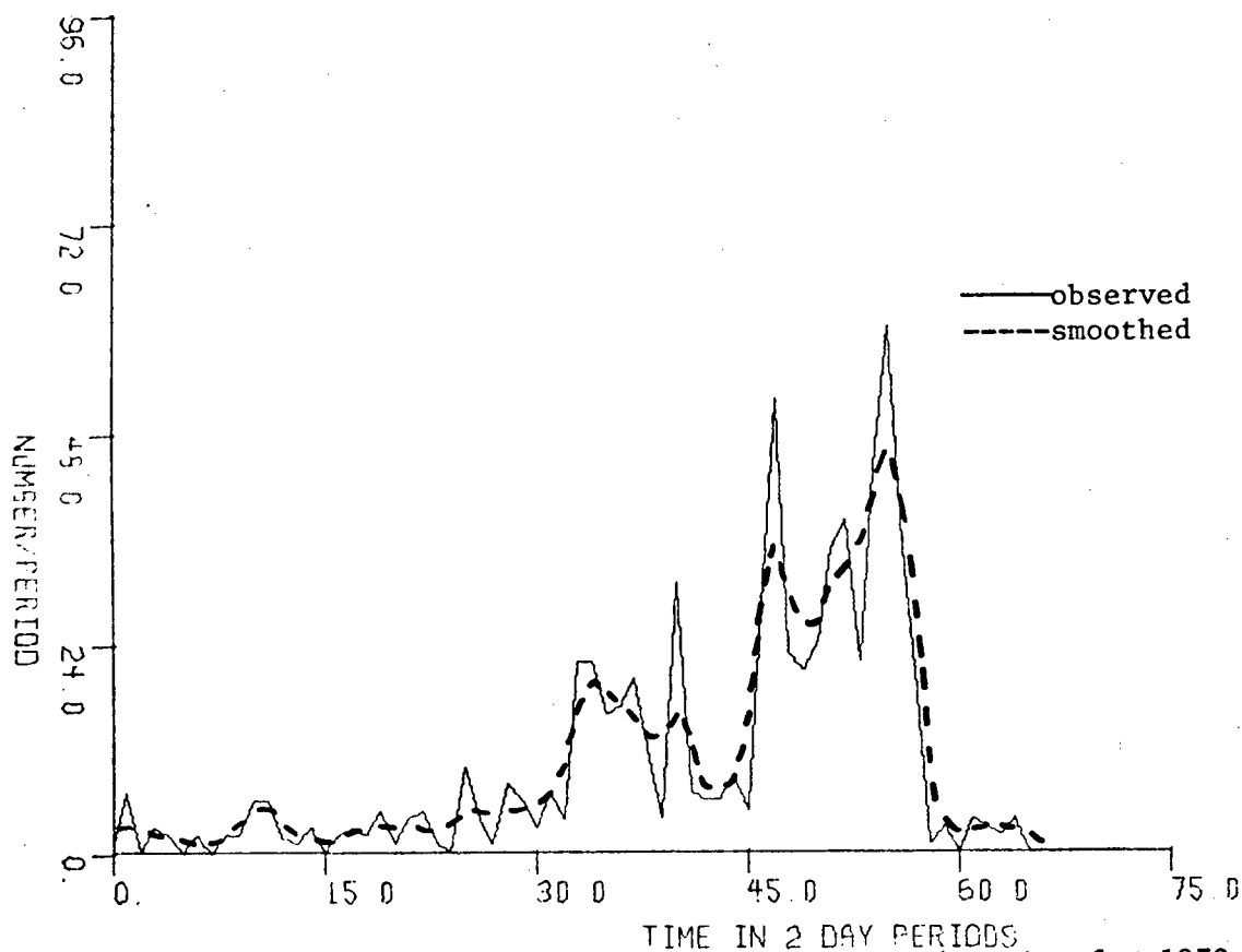
Fig. 2. Observed series vs. smoothed series for 1970 data
