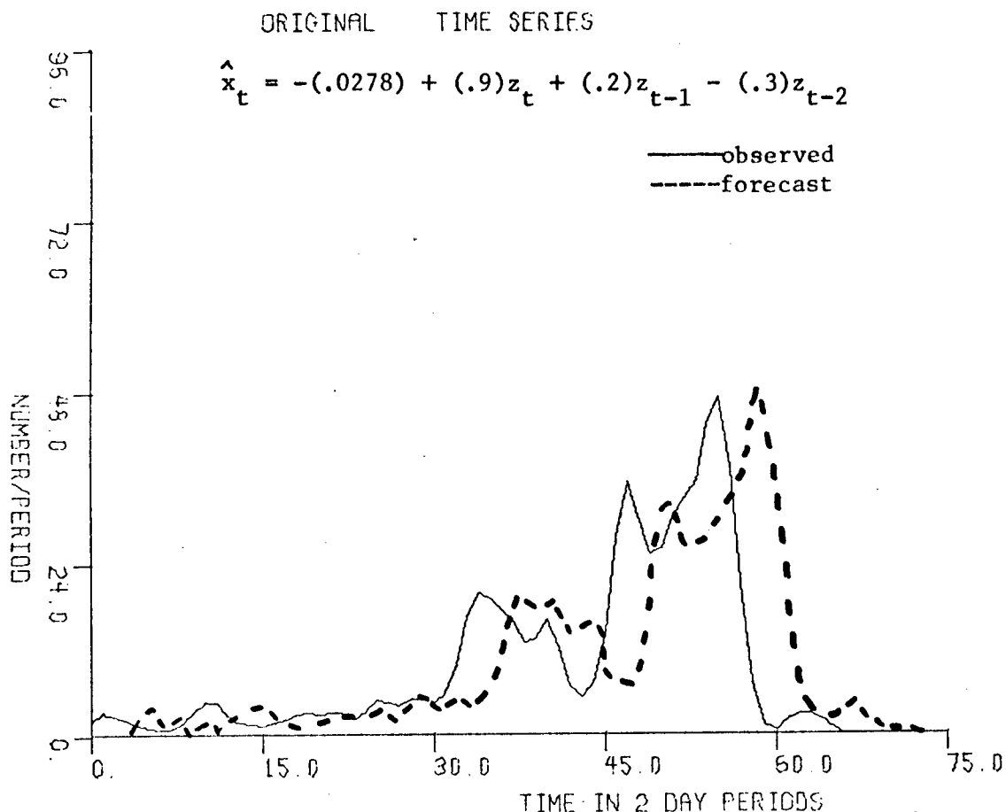
Fig. 5 Observed vs. 4-day ahead forecast series for 1970 smoothed data.
