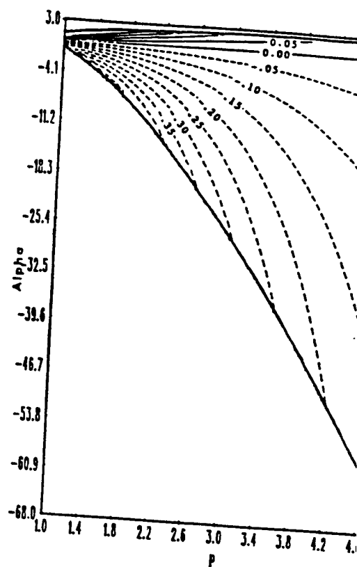
FIGURE 15 Contour Graph of \rho as a function of p and \alpha_p for Density (9) Constructed from N(0,1)
