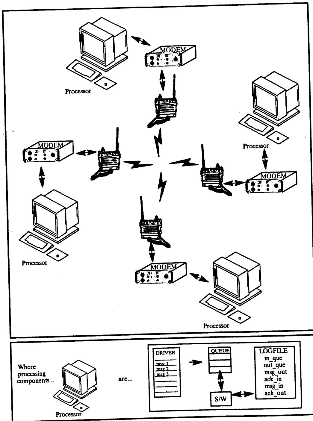
Figure 1. Experiment Configuration.
