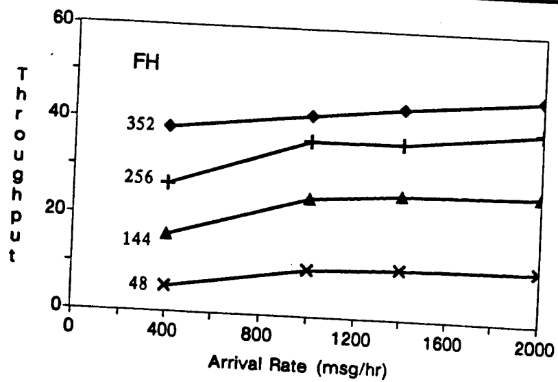
Figure 8. Normalized Throughput vs Arrival Rate Grouped by Message Length (Frequency Hopping)
