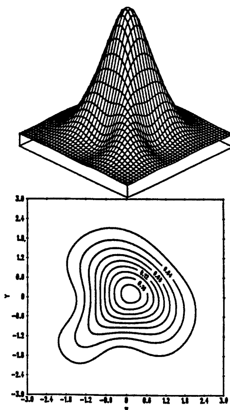
FIGURE 21 Density (10) Constructed from N(0,1) , Preserving the Margins, (\alpha_1, \alpha_2) = (-1.0, 2.90) , \rho = -0.06
